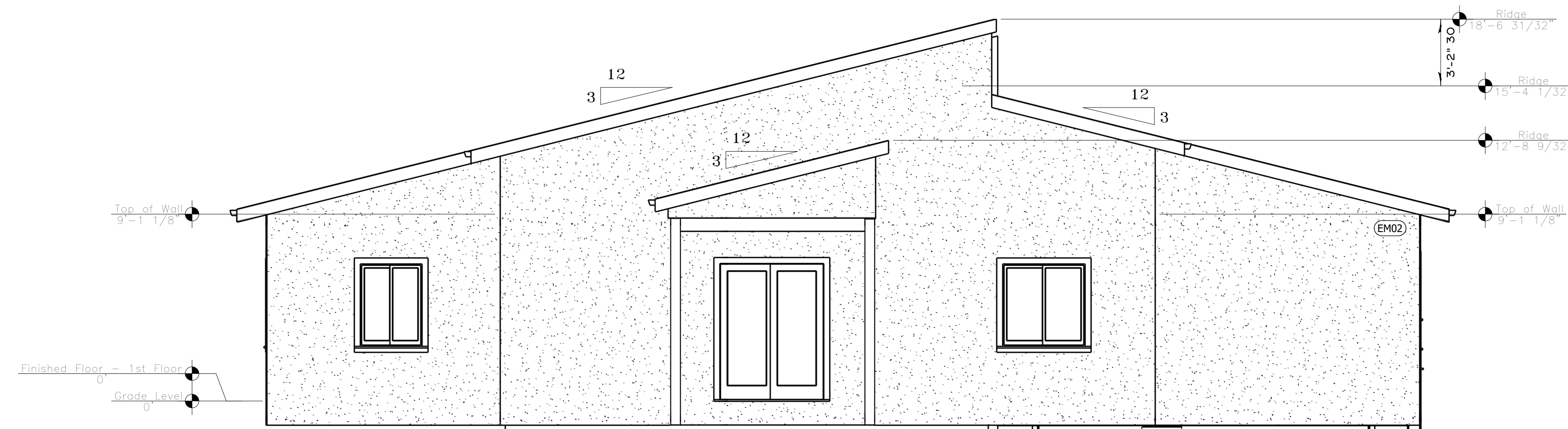
E4 Back Elevation Scale = N/A
