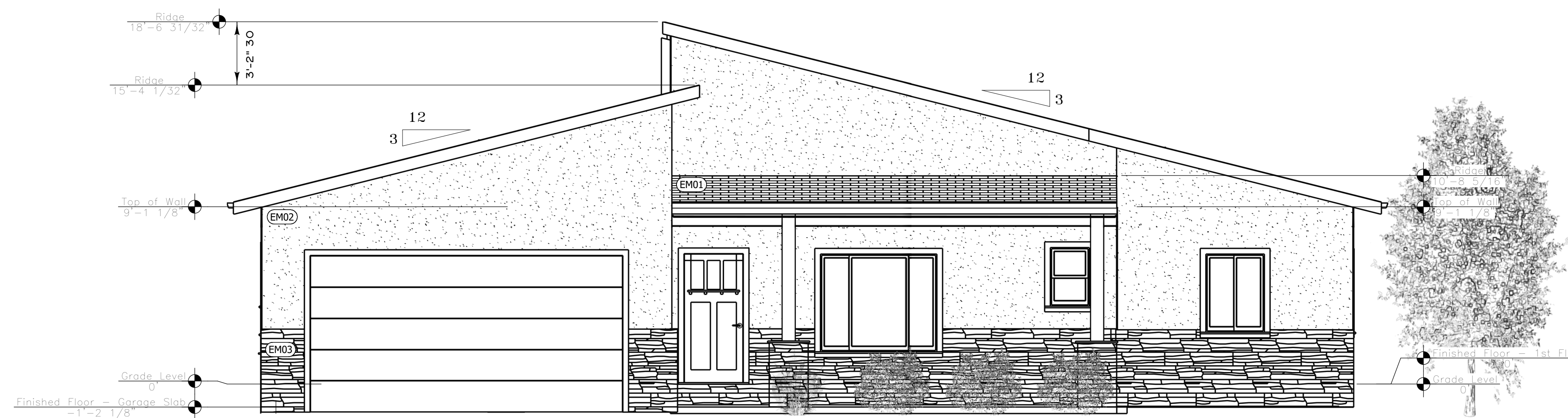
E3 Front Elevation Scale = N/A
